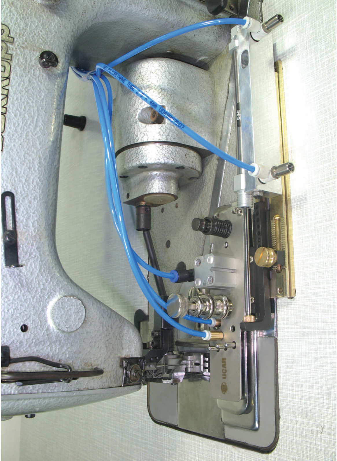
HAVALI KUMAFI BİRLİKTE RME APARATI (ZIPPY)
